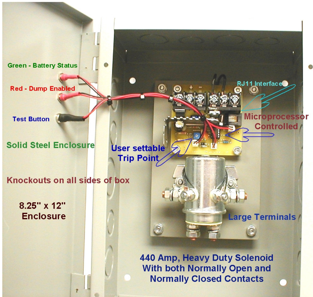
Coleman Air - C440 XL 440 Amp Diversion Controller
